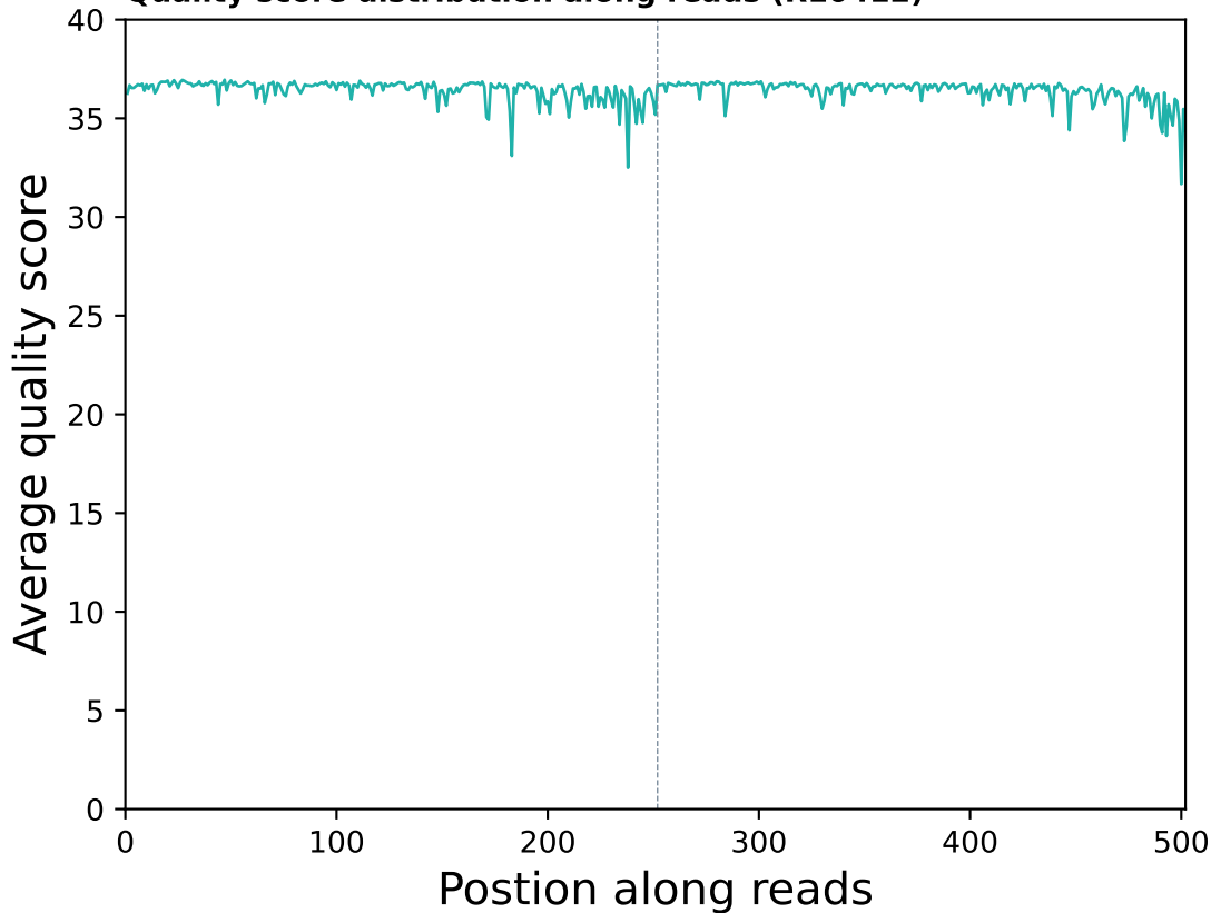
Quality score distribution along reads (R10412)
